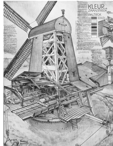
Paltrokmolen tek.A. Sipman 1943
